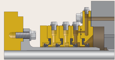
Cross-section SUPREME SG
