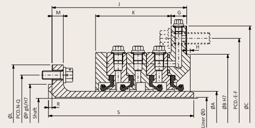
Cross-section SUPREME SG
